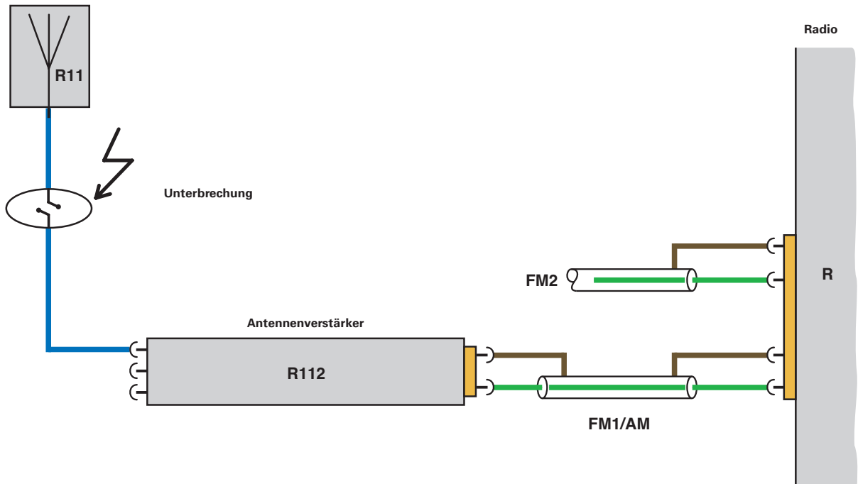
Antenne (AM/FM1)
